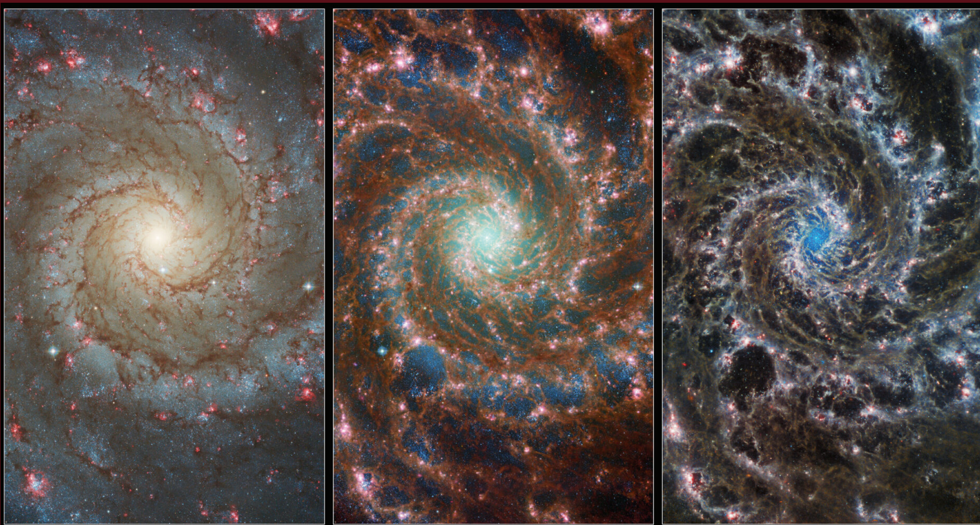
Hubble / Optical
